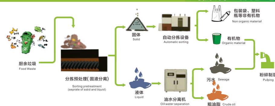
PROCESS FLOW OF LARGE WASTE TREATMENT 餐厨/厨余垃圾处理工艺流程
