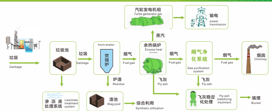
GARBAGE INCINERATION POWER FLOW CHART 垃圾焚烧发电示意图
