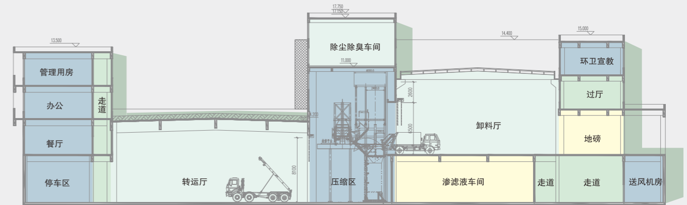
Large garbage compression and transfer station
